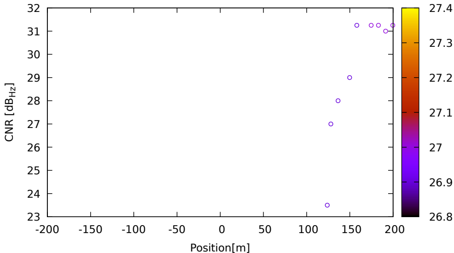
CNR vs position for G09 (L5) on Xiaomi11T - DOY 262 jam. 1
