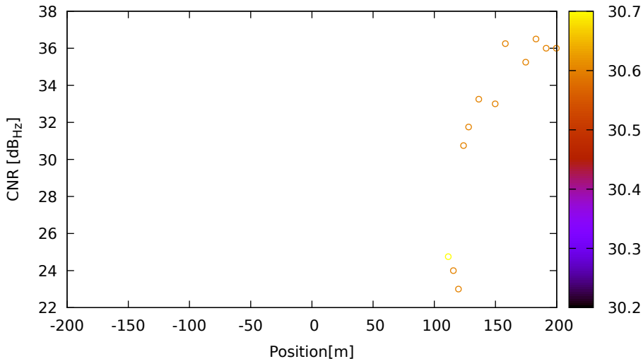
CNR vs position for G21 (L1) on Xiaomi11T - DOY 262 jam. 1
