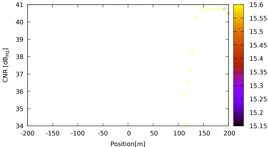
CNR vs position for G22 (L1) on Xiaomi11T - DOY 262 jam. 1
