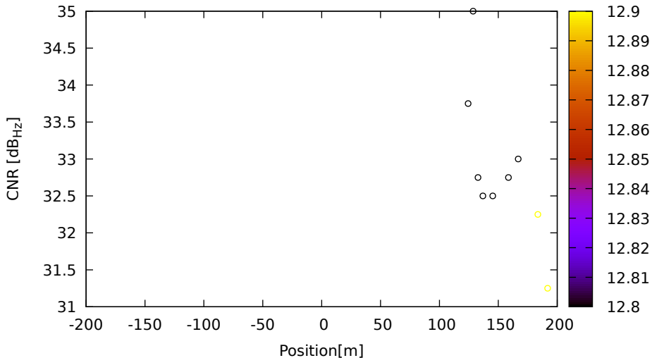
CNR vs position for C26 (B1) on XiaomiMi8 - DOY 262 jam. 1
