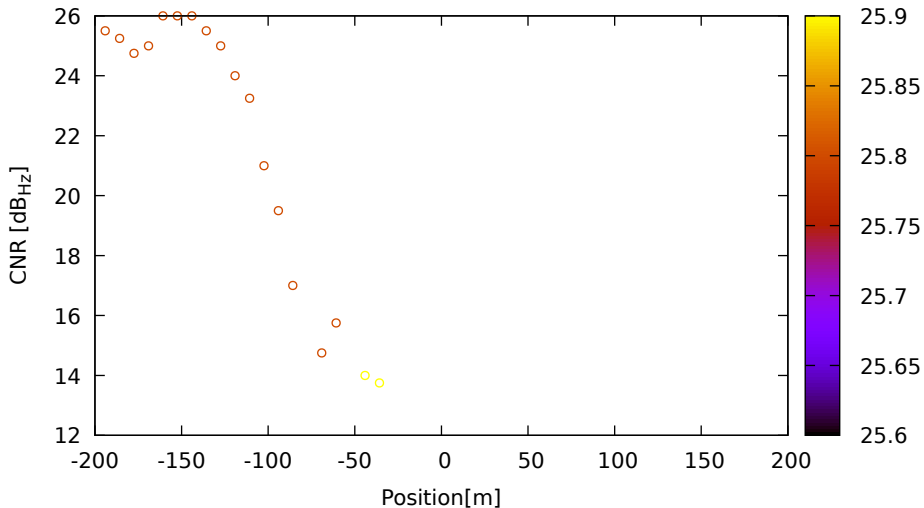
CNR vs position for E03 (E1) on XiaomiMi8 - DOY 262 jam. 2
