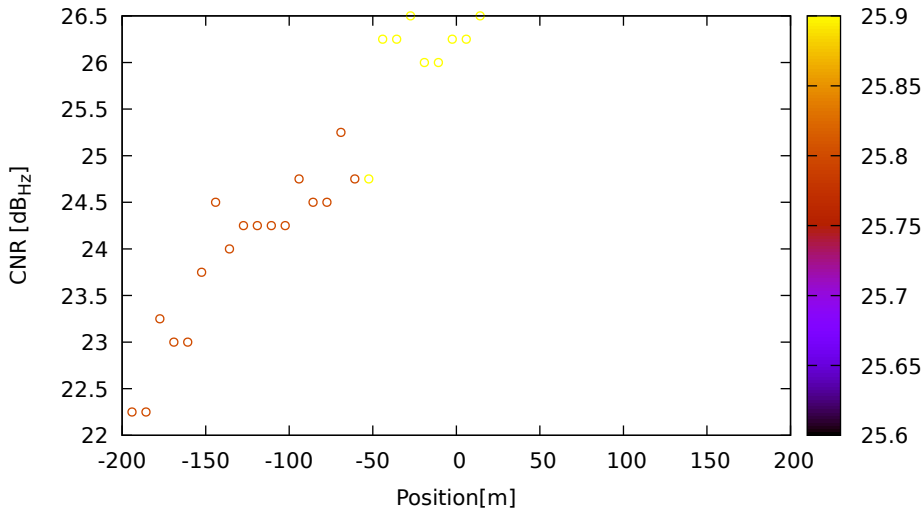
CNR vs position for E03 (E5a) on XiaomiMi8 - DOY 262 jam. 2
