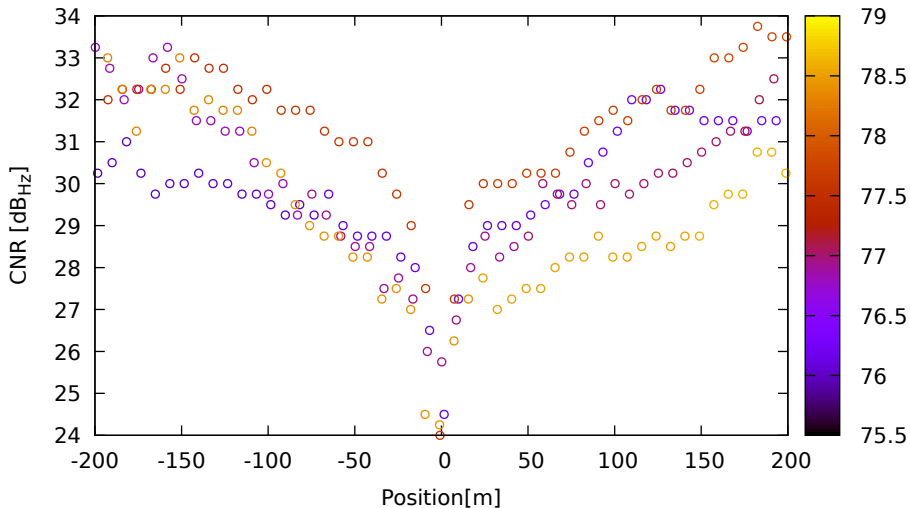
CNR vs position for E05 (E1) on XiaomiMi8 - DOY 262 jam. 1
