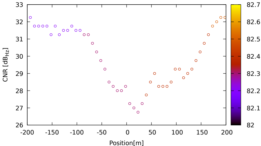
CNR vs position for E05 (E1) on XiaomiMi8 - DOY 262 jam. 3
