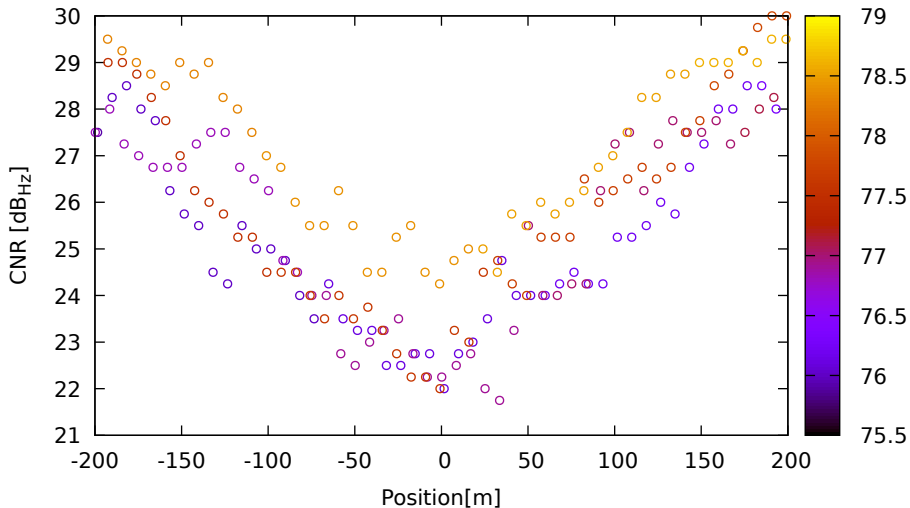
CNR vs position for E05 (E5a) on XiaomiMi8 - DOY 262 jam. 1
