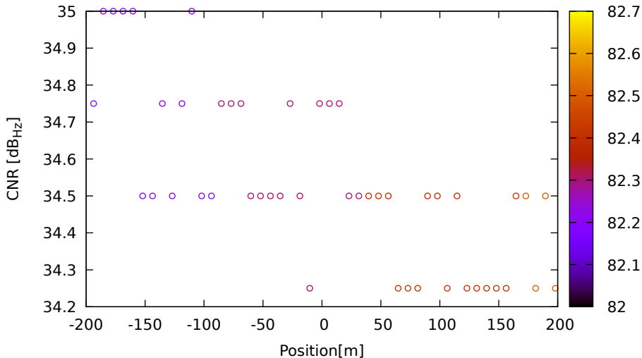
CNR vs position for E05 (E5a) on XiaomiMi8 - DOY 262 jam. 3
