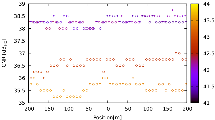
CNR vs position for E09 (E5a) on XiaomiMi8 - DOY 262 jam. 2
