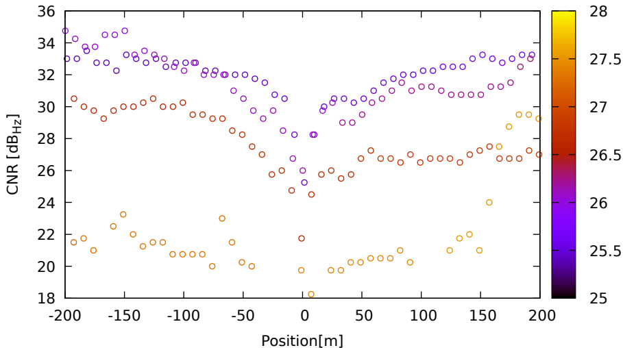
CNR vs position for E15 (E1) on XiaomiMi8 - DOY 262 jam. 1
