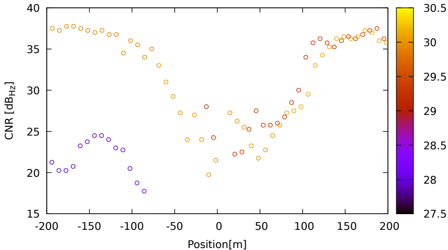
CNR vs position for E15 (E1) on XiaomiMi8 - DOY 262 jam. 2
