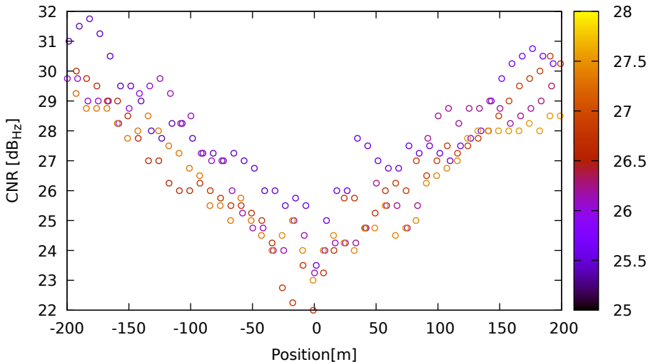
CNR vs position for E15 (E5a) on XiaomiMi8 - DOY 262 jam. 1
