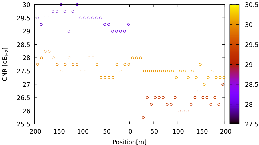
CNR vs position for E15 (E5a) on XiaomiMi8 - DOY 262 jam. 2
