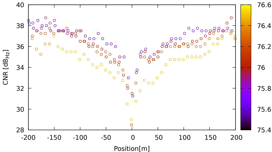
CNR vs position for E34 (E1) on XiaomiMi8 - DOY 262 jam. 1
