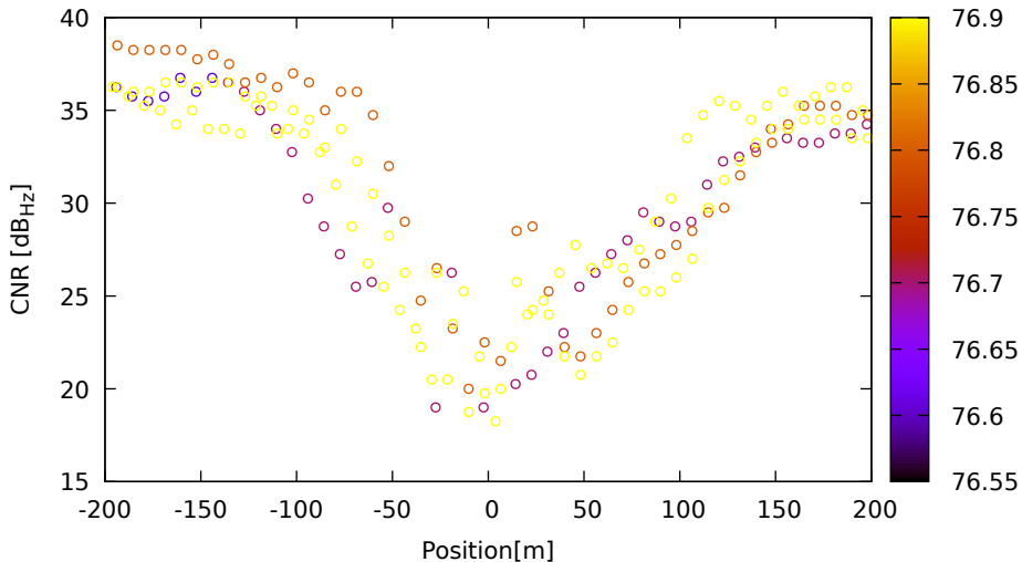
CNR vs position for E34 (E1) on XiaomiMi8 - DOY 262 jam. 2
