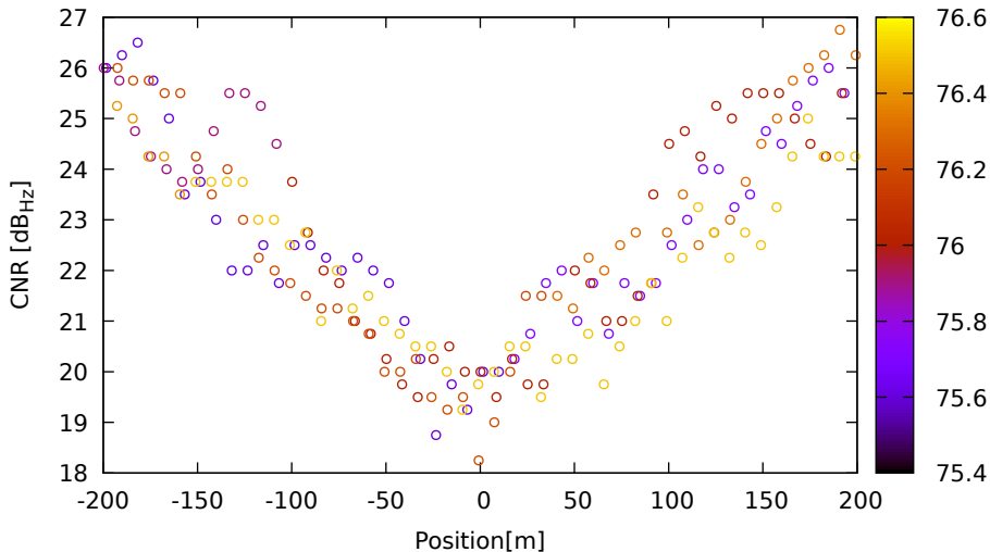
CNR vs position for E34 (E5a) on XiaomiMi8 - DOY 262 jam. 1
