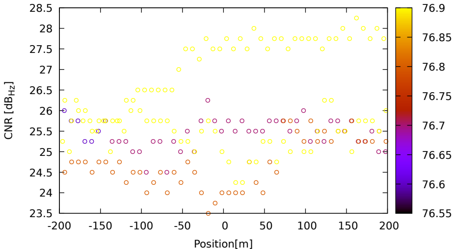
CNR vs position for E34 (E5a) on XiaomiMi8 - DOY 262 jam. 2
