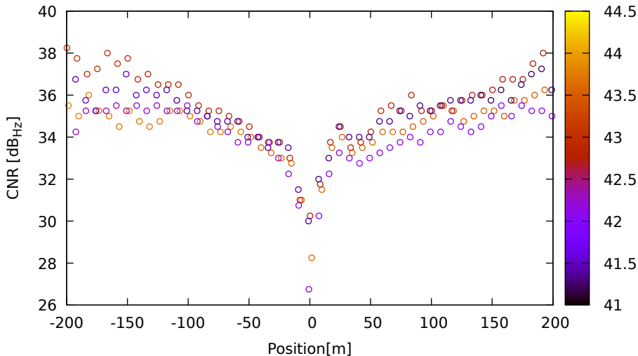
CNR vs position for E36 (E1) on XiaomiMi8 - DOY 262 jam. 1
