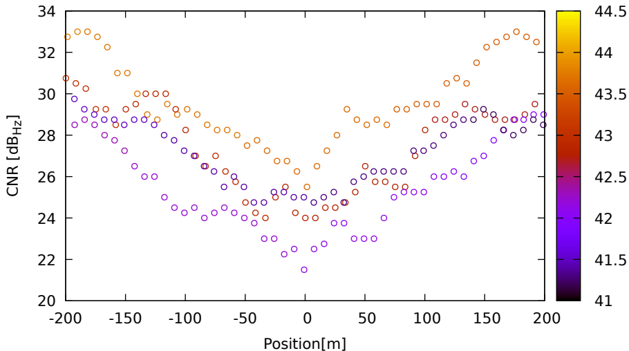
CNR vs position for E36 (E5a) on XiaomiMi8 - DOY 262 jam. 1
