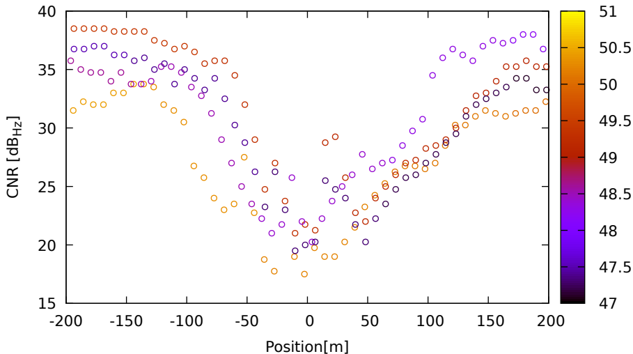
CNR vs position for G01 (L1) on XiaomiMi8 - DOY 262 jam. 2
