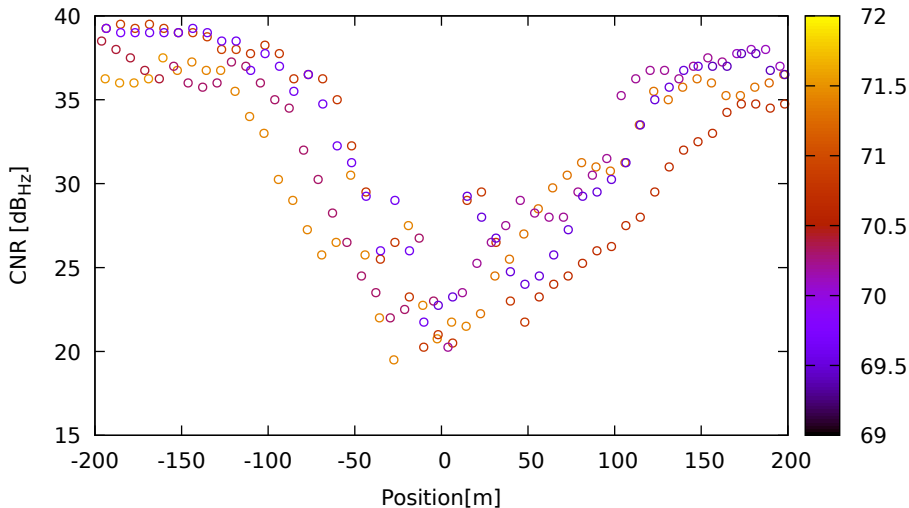
CNR vs position for G03 (L1) on XiaomiMi8 - DOY 262 jam. 2
