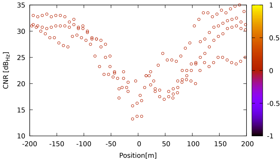
CNR vs position for G06 (L1) on XiaomiMi8 - DOY 262 jam. 2
