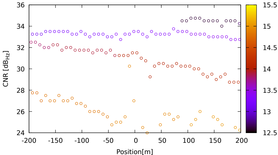
CNR vs position for G06 (L5) on XiaomiMi8 - DOY 262 jam. 2
