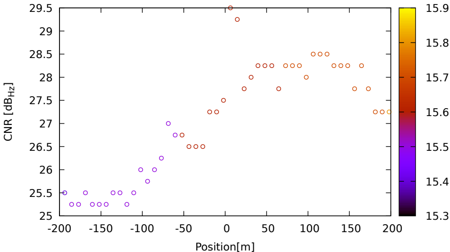
CNR vs position for G06 (L5) on XiaomiMi8 - DOY 262 jam. 3
