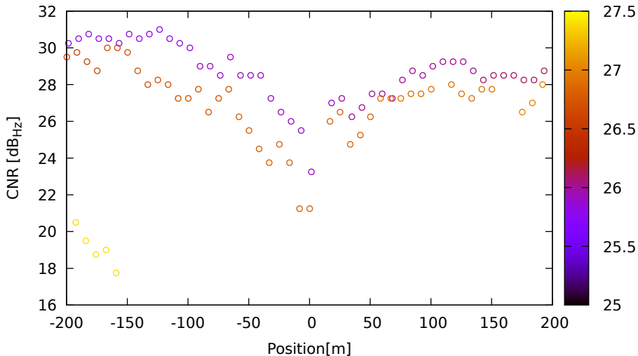
CNR vs position for G09 (L1) on XiaomiMi8 - DOY 262 jam. 1
