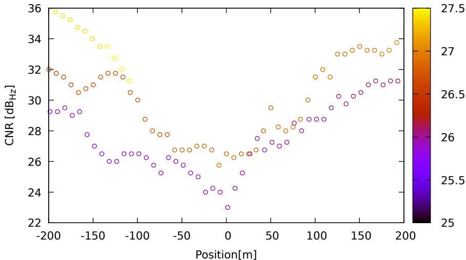
CNR vs position for G09 (L5) on XiaomiMi8 - DOY 262 jam. 1
