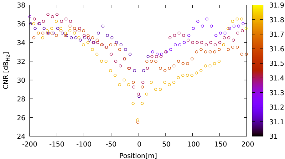
CNR vs position for G19 (L1) on XiaomiMi8 - DOY 262 jam. 1
