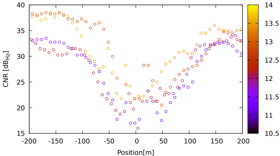
CNR vs position for G22 (L1) on XiaomiMi8 - DOY 262 jam. 2
