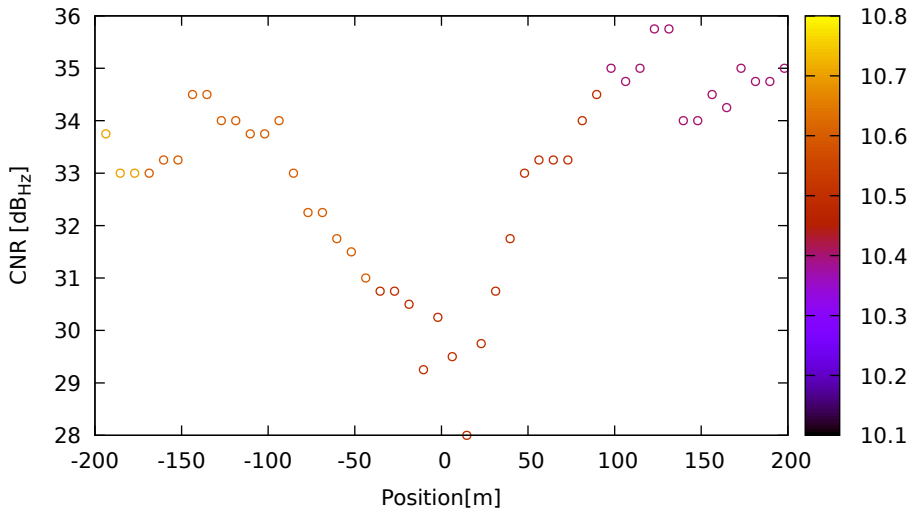
CNR vs position for G22 (L1) on XiaomiMi8 - DOY 262 jam. 3
