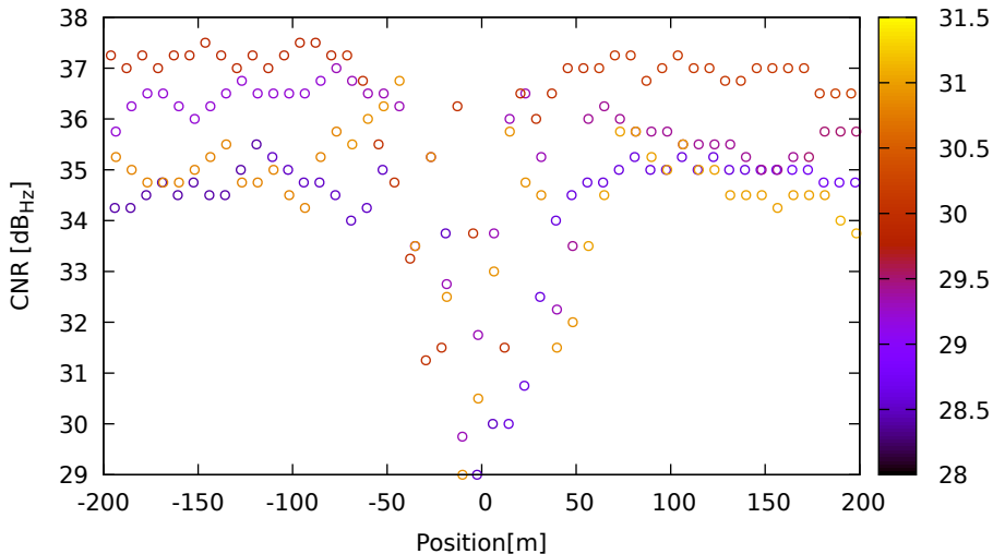
CNR vs position for R02 (G1) on XiaomiMi8 - DOY 262 jam. 2
