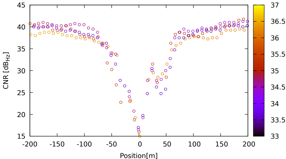
CNR vs position for R08 (G1) on XiaomiMi8 - DOY 262 jam. 1
