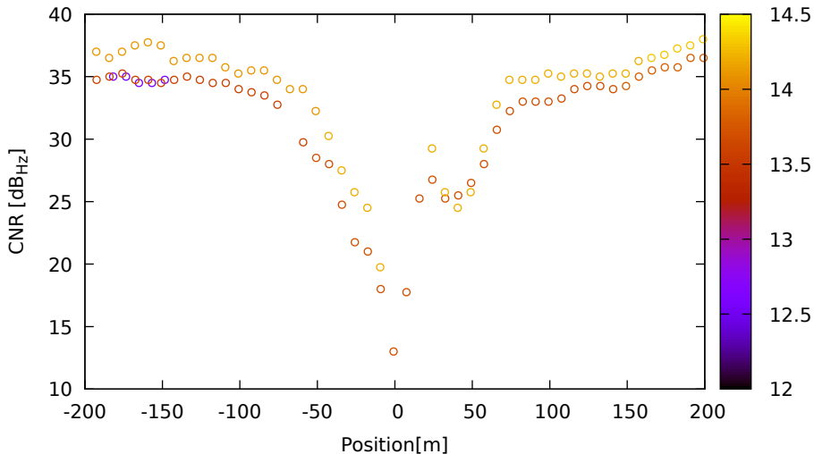
CNR vs position for R10 (G1) on XiaomiMi8 - DOY 262 jam. 1
