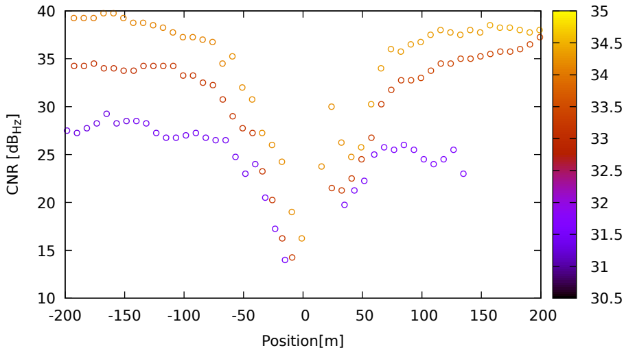
CNR vs position for R17 (G1) on XiaomiMi8 - DOY 262 jam. 1
