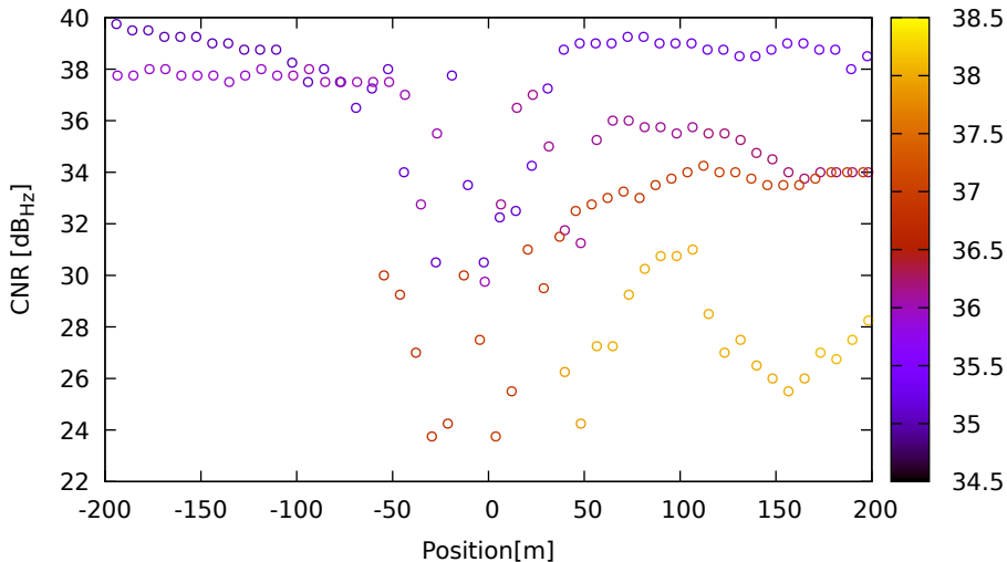
CNR vs position for R17 (G1) on XiaomiMi8 - DOY 262 jam. 2
