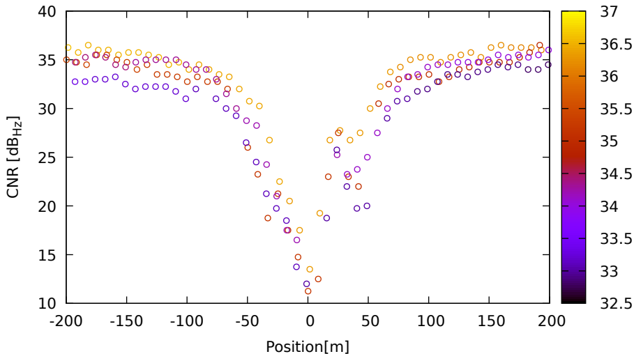
CNR vs position for R23 (G1) on XiaomiMi8 - DOY 262 jam. 1
