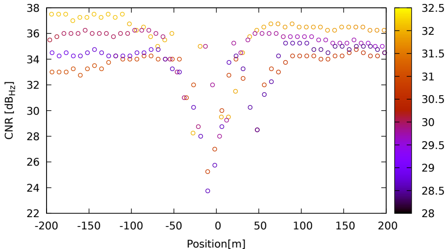
CNR vs position for R23 (G1) on XiaomiMi8 - DOY 262 jam. 2
