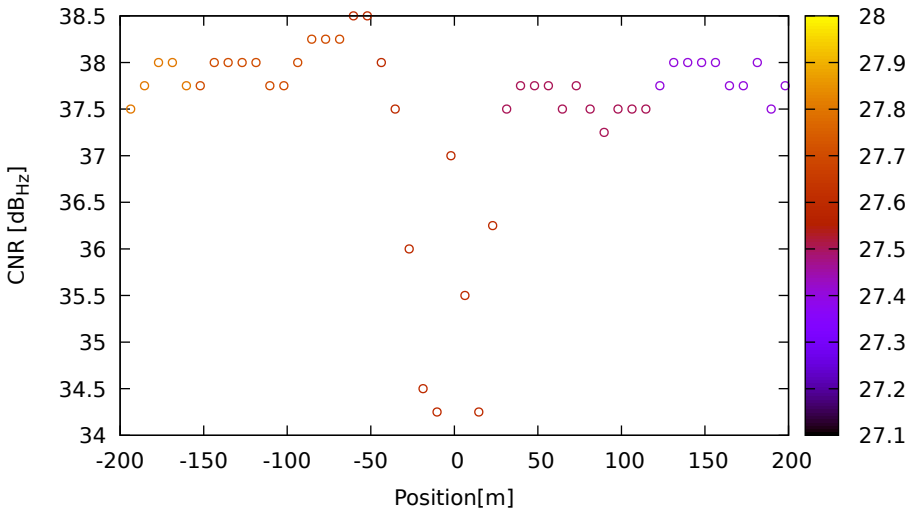
CNR vs position for R23 (G1) on XiaomiMi8 - DOY 262 jam. 3
