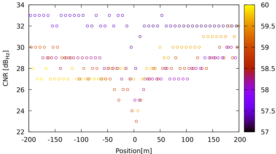
CNR vs position for C11 (B1) on HuaweiP40 - DOY 263 jam. 2
