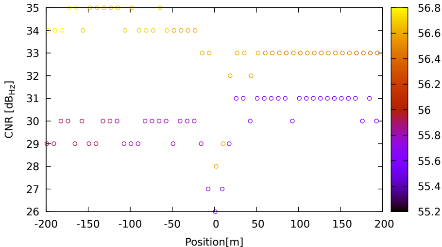
CNR vs position for C11 (B1) on HuaweiP40 - DOY 263 jam. 3
