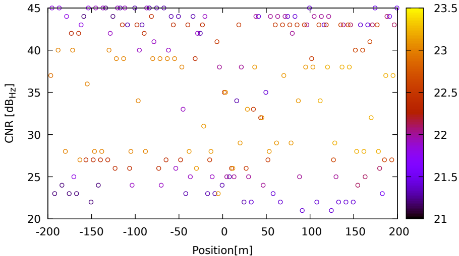
CNR vs position for C28 (B1) on HuaweiP40 - DOY 263 jam. 2
