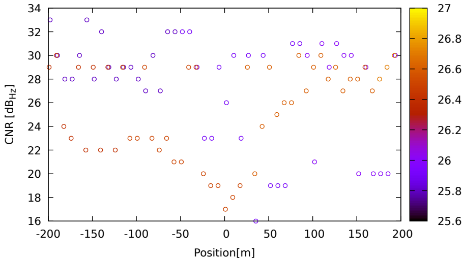
CNR vs position for C33 (B1) on HuaweiP40 - DOY 263 jam. 3
