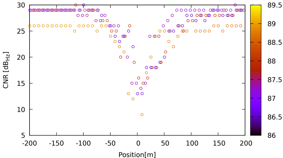
CNR vs position for E12 (E1) on HuaweiP40 - DOY 263 jam. 1
