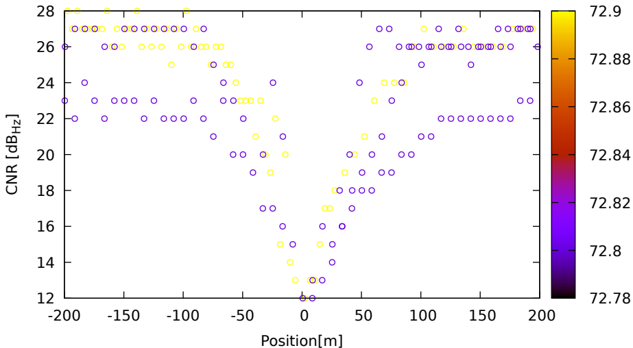
CNR vs position for E19 (E1) on HuaweiP40 - DOY 263 jam. 1
