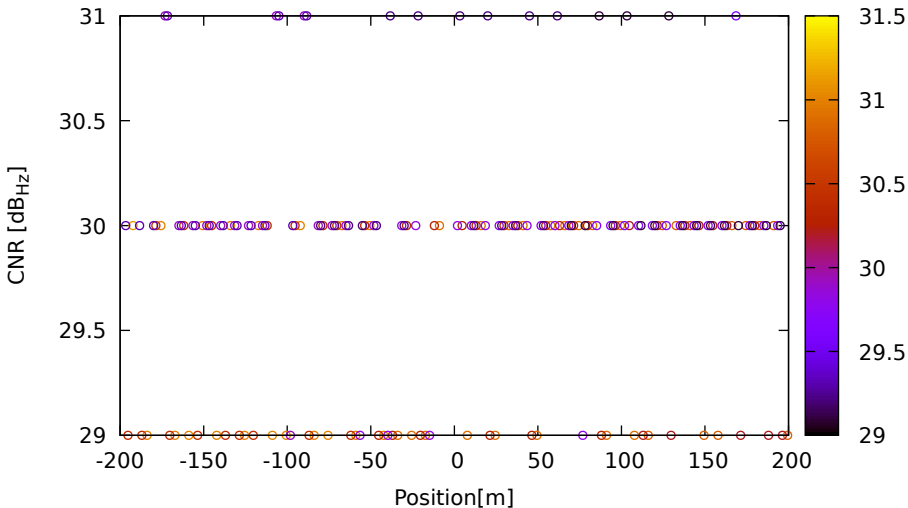
CNR vs position for E33 (E1) on HuaweiP40 - DOY 263 jam. 2
