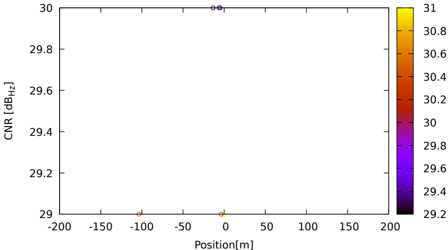
CNR vs position for E33 (E5a) on HuaweiP40 - DOY 263 jam. 2
