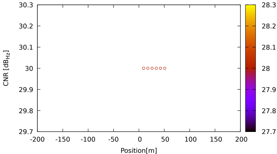
CNR vs position for E33 (E5a) on HuaweiP40 - DOY 263 jam. 3
