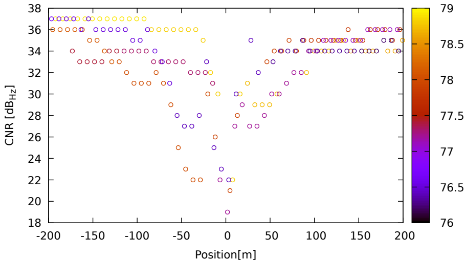
CNR vs position for G01 (L1) on HuaweiP40 - DOY 263 jam. 2
