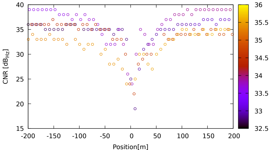
CNR vs position for G04 (L1) on HuaweiP40 - DOY 263 jam. 1
